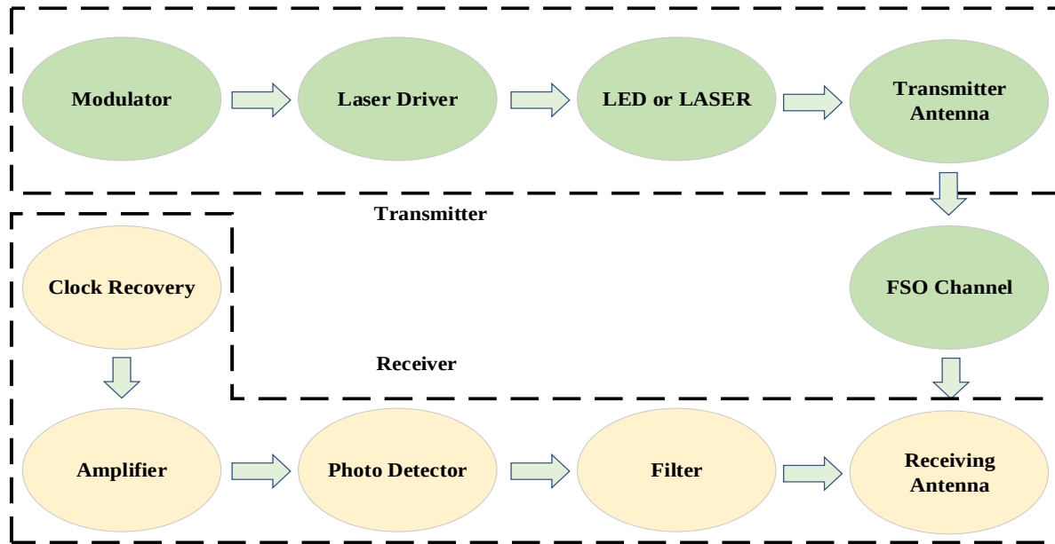
Figure 1. FSO system block diagram
