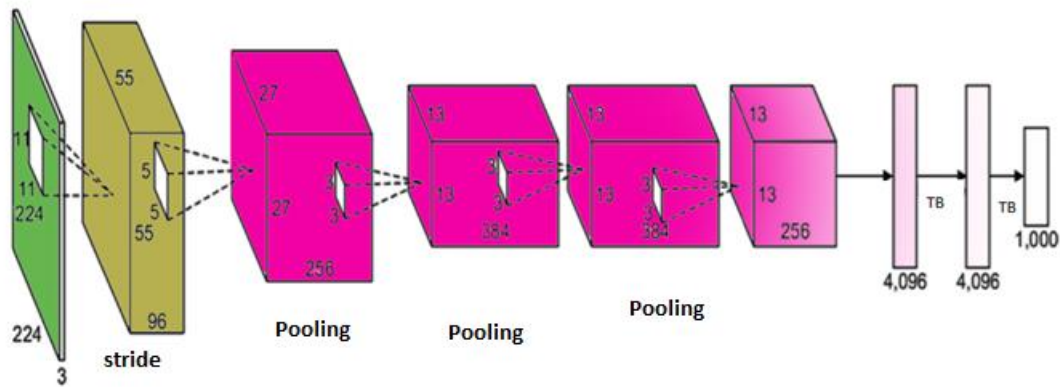
Figure 1. Model Architecture [1]
