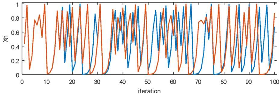
Fig. 1 Logistic map output for very close different initial conditions
