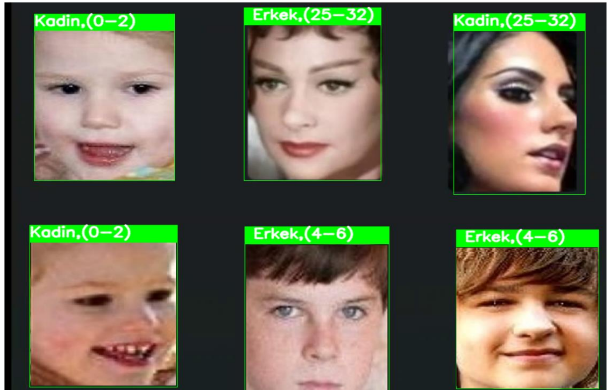
Figure 5. Dataset Outputs
