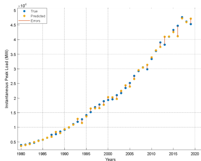
Figure 4. Error graph between real and predicted values using ANN
