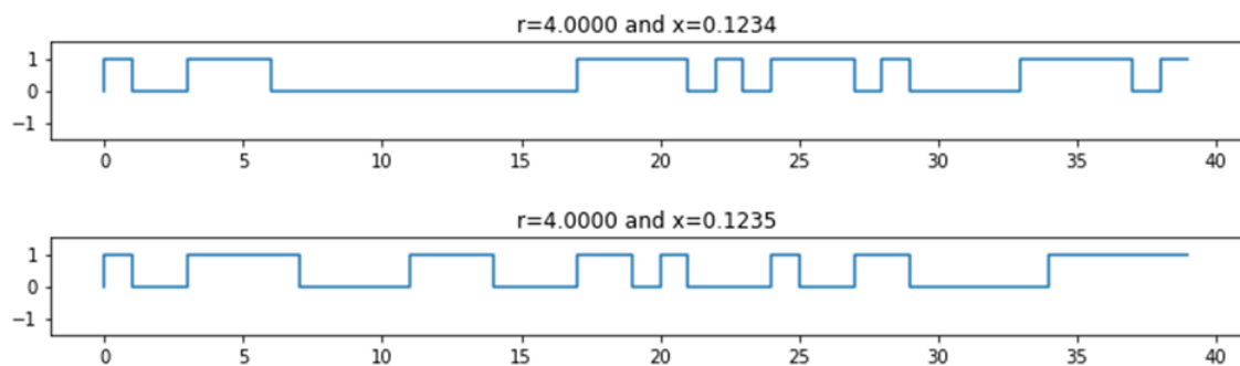
Fig. 3 Generated encryption key for different initial values
