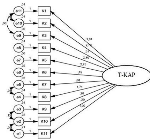
Figure 1: The Path Diagram of the Confirmatory Factor Analysis
