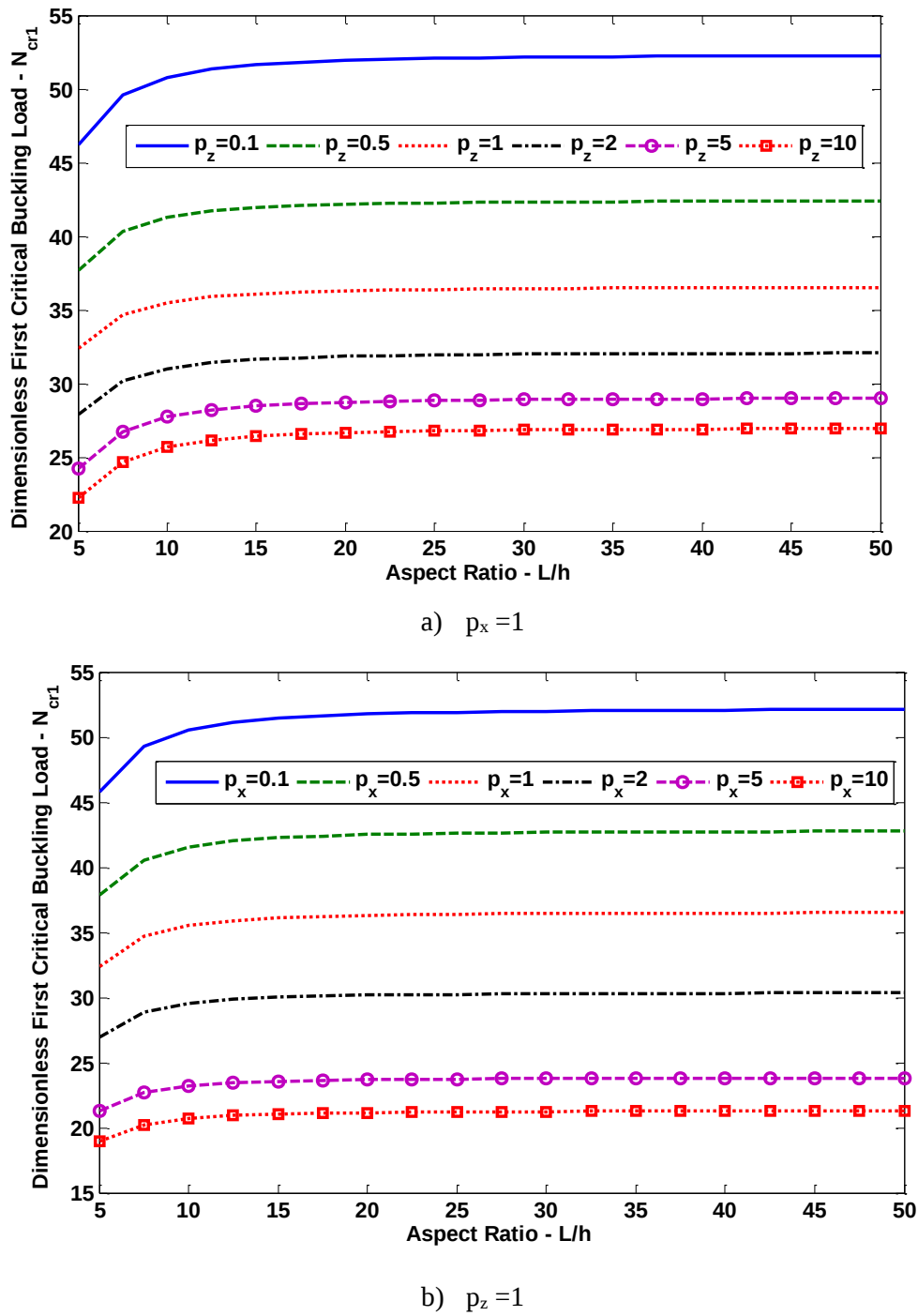
Figure 7. Variation of the dimensionless first critical buckling loads of CS two directional FGBs with respect to variation of gradient indexes and aspect ratios a) p_x = 1 and b) p_z = 1
