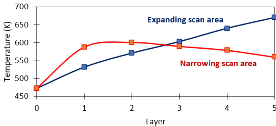
Figure 8. The temperature stored on 1 st layer during scanning of 5 layers for narrowing and expanding parts
