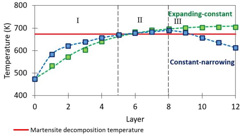
Figure 9. The temperature stored on 1 st layer during scanning of 12 layers for expanding-constant and constant-narrowing parts
