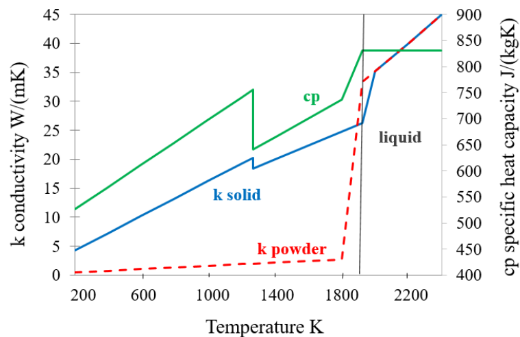
Figure 3. Thermal conductivity and specific heat capacity properties for Ti6Al4V
