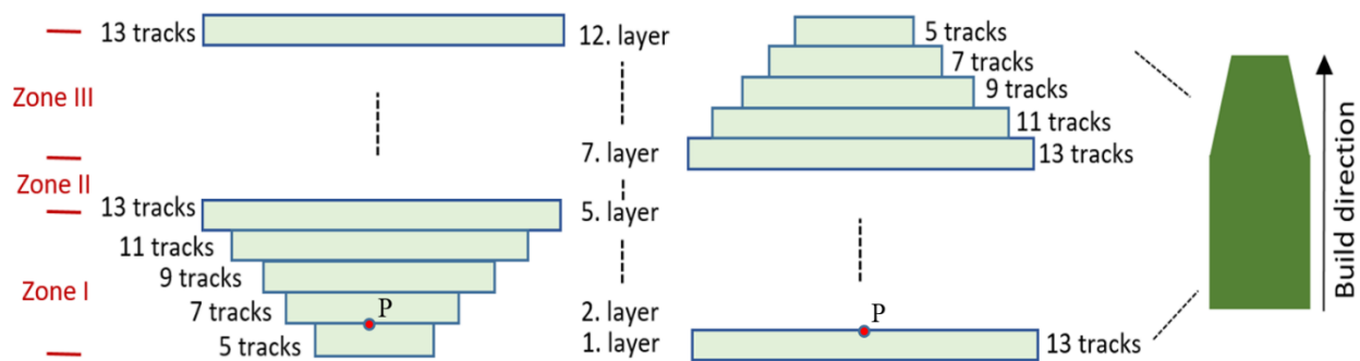
Figure 6. The build orientation of expanding-constant (a) and constant-narrowing (b) parts
