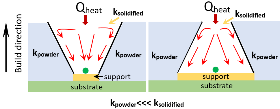
Figure 2. The heat conduction within the part in different orientations in LPBF
