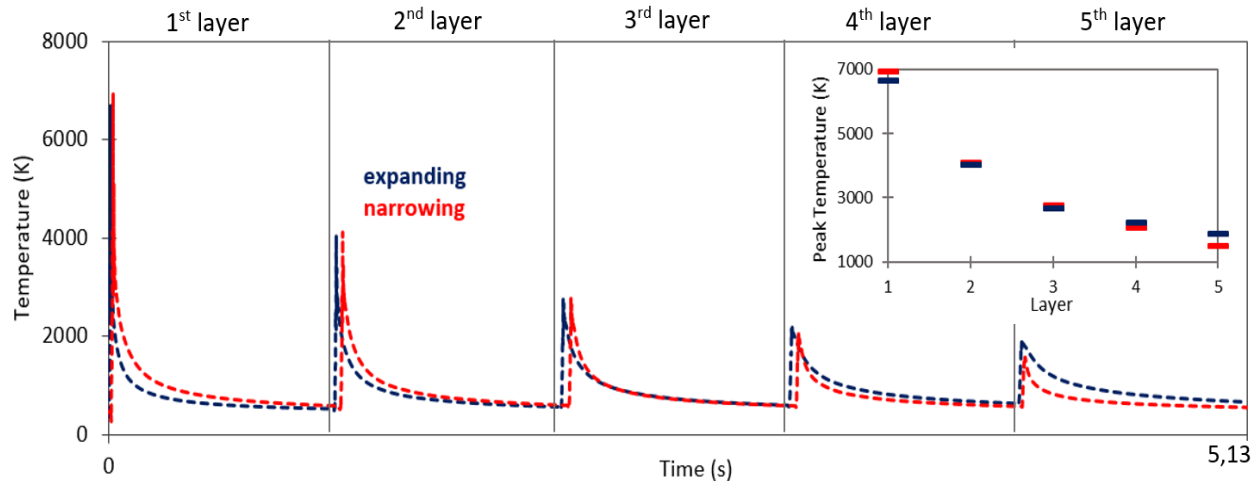
Figure 7. The temperature of P point on the 1 st layer during scanning of 5 subsequent layers for narrowing and expanding parts
