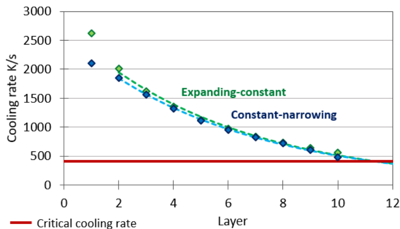
Figure 10. The cooling rate of 1 st layer during scanning of 12 layers for expanding-constant and constant-narrowing parts
