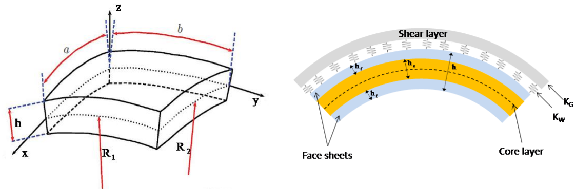
(a) : Configuration and coordinate system of CNT-RSSC shell
