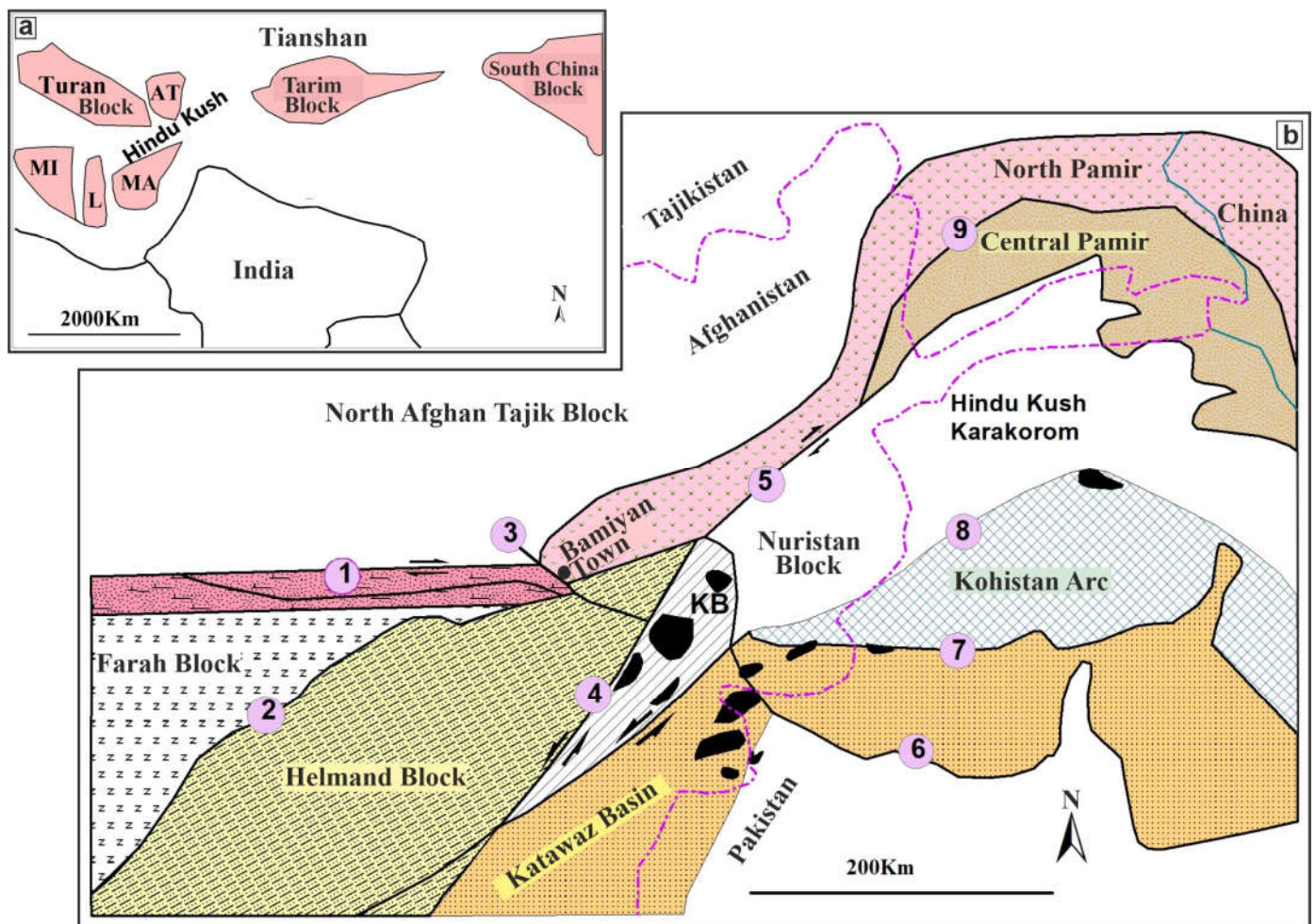
Fig. 4. (a) Current location of Precambrian blocks in South Asia (AT- Afghan-Tajik block, MA-Central Afghan Blocks, MI- Central Iranian Block, L-Lut Block, South China Block, Turan Block, [29]. (b) Tectonic map of Afghanistan - Western Himalaya - Hindu Kush region [11], [13], [26], [30], [31]. The black areas in the Kabul Block (NW) are ophiolite formations. 1-Harirod Fault (Paleozoic Suture), 2-Helmand Fault (Mesozoic Suture), 3-Bamiyan-Shibar Fault, 4-Chaman Fault, 5-Panjshir Fault, 6-Main Boundary Thrust (Indus-Tsangpo Suture), 8-Shyok Suture, 9-Mesozoic Suture
