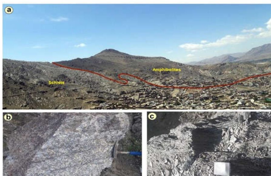
Fig. 18. a) Amphibolites and schists observed in the Welayeti formation, a) Amphibolite, b) Garnet-staurolite-schists, c) Micaschists. Location: Chehelston mountains
