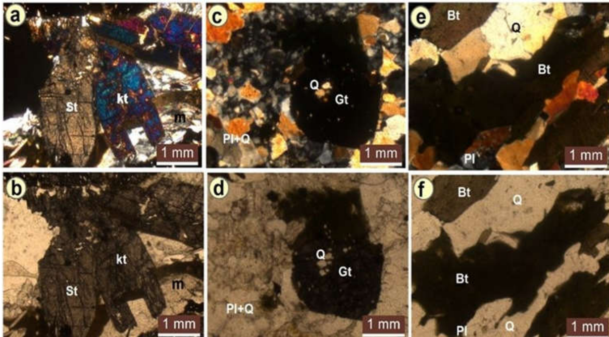
Fig 19. The microscopic view of different schist ralted to Welayeti formation, garnet perfiroblasts and kyanite and staurolite are seen, a, b) kyanite-garnet-staurolite mica schist, c, d) garnet mica schist, e, f) mica schist, a, c, e) /nicol, b, d, f) / nicol. St: staurolite, Gt: garnet, Pl: plagioclase, Q: quartz, Bt: biotite, kt: kyanite
