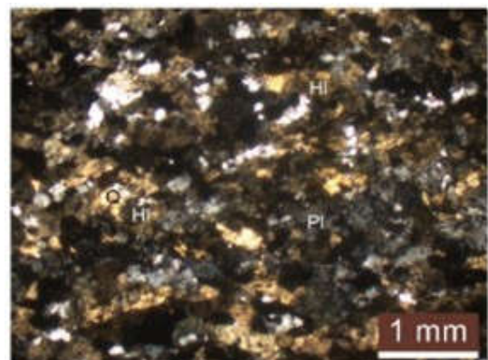
Fig. 13. Amphibole gneisses observed in the Sherdarwaza formation. // Nicol, Q: Quartz, Pl: Plagioclase, Hl: Hornblende
