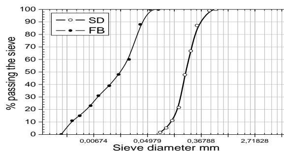
Figure 1. The grading curves of the aggregates.
