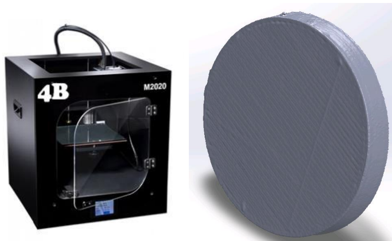
Figure 1. (a) FDM machine used to produce the samples, (b) PLA sample.
