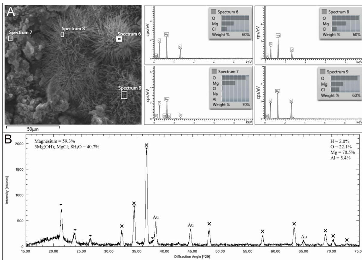
Figure 6. Compositional analysis of AZ31 plate immersed in 3.5% sodium chloride solution: A) EDX analysis results from an area imaged with a BSE detector (spectra depict weight ratios), B) Quantitative XRD analysis results (percentages of the compounds and elements are based on weight).
