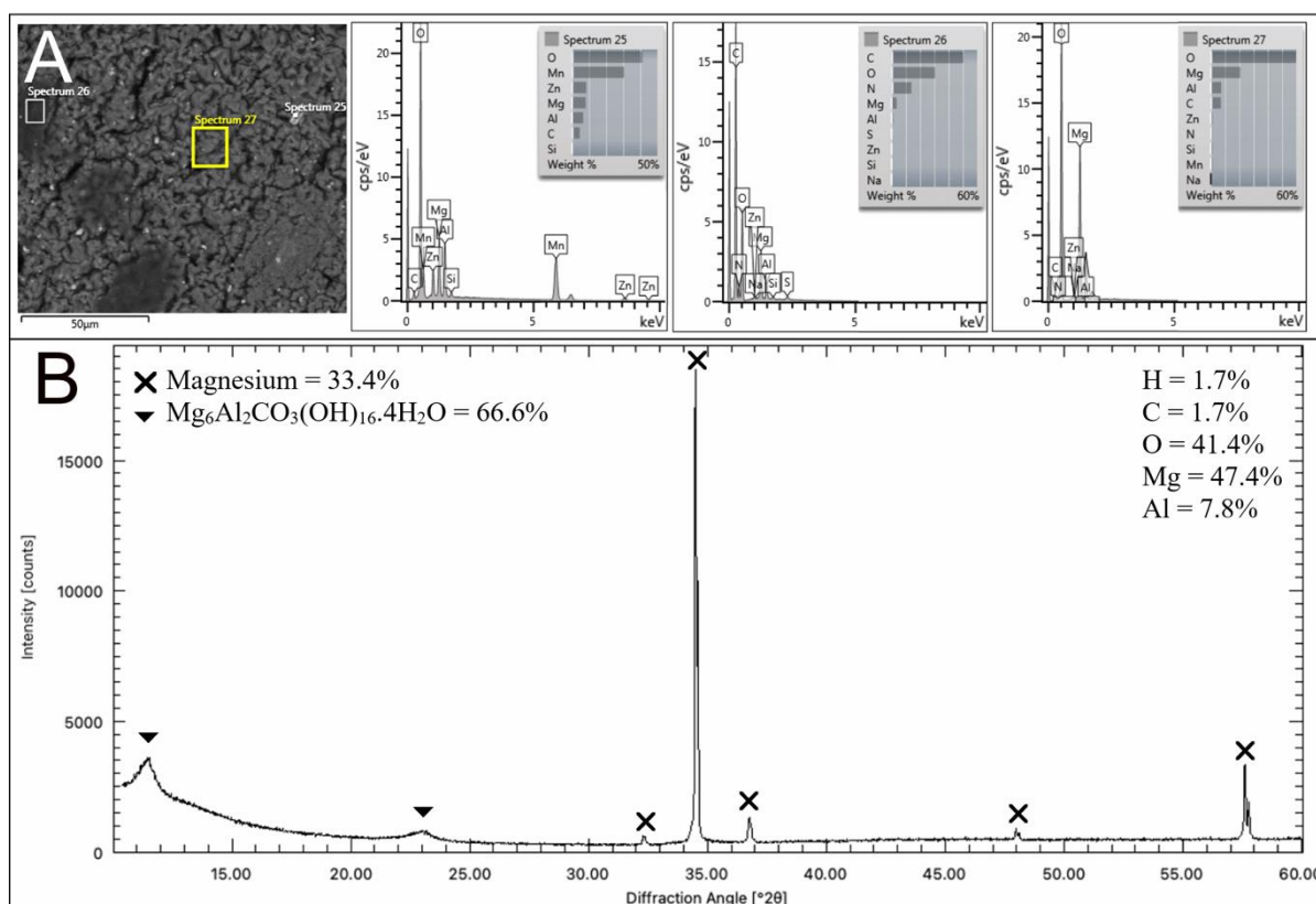
Figure 4. Compositional analysis of AZ31 samples immersed in DIW for 21 days: A) EDX analysis results from an area imaged with a BSE detector (spectra depict weight ratios), B) Quantitative XRD analysis results (percentages of the compounds and elements are based on weight).
