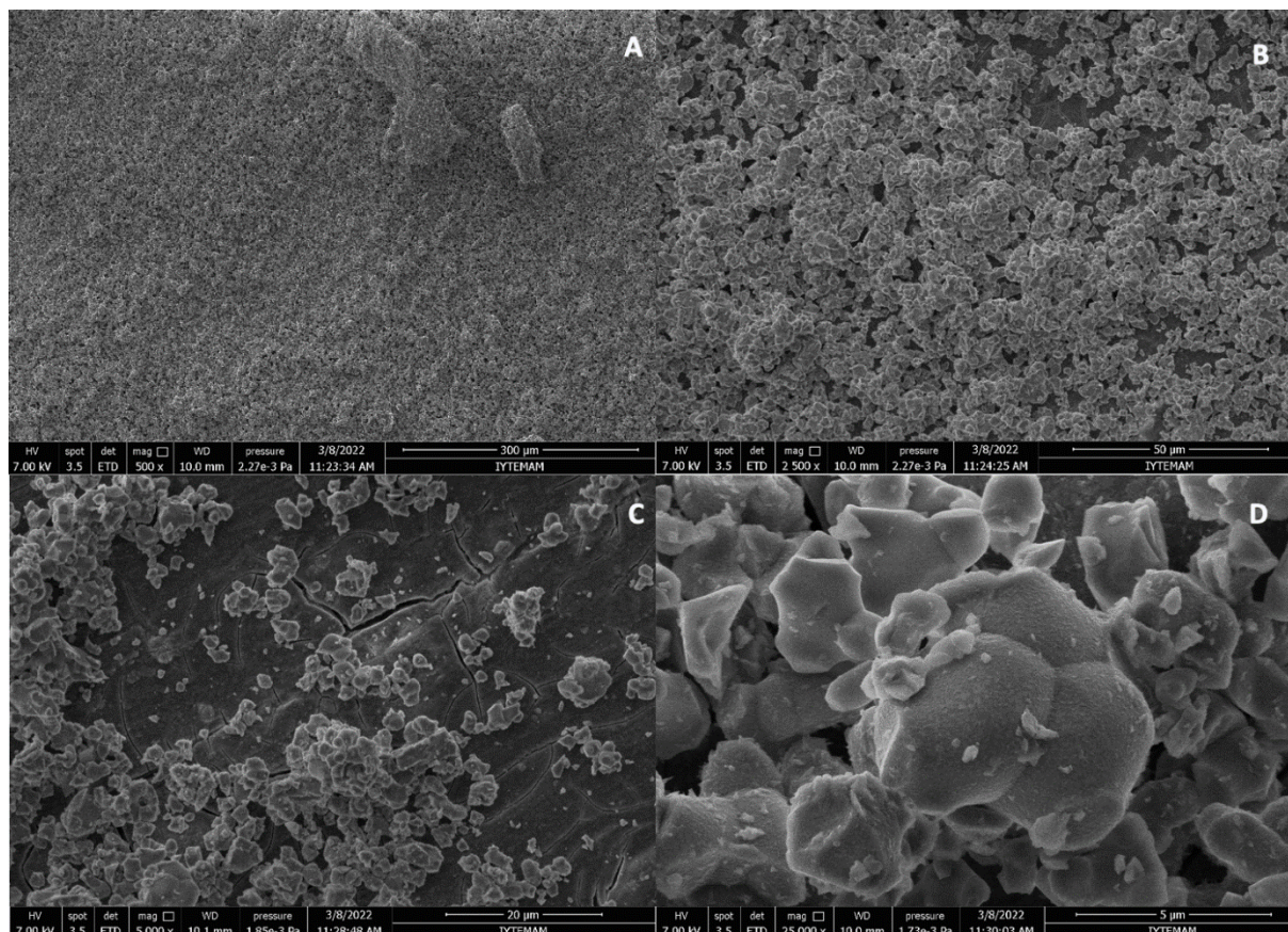
Figure 14. Surface morphology of AZ31 sample immersed in saturated TCP solution for 21 days, imaged using a SE detector at a magnification of: (A) 500X, (B) 2500X, (C) 5000X, (D) 25000X.
