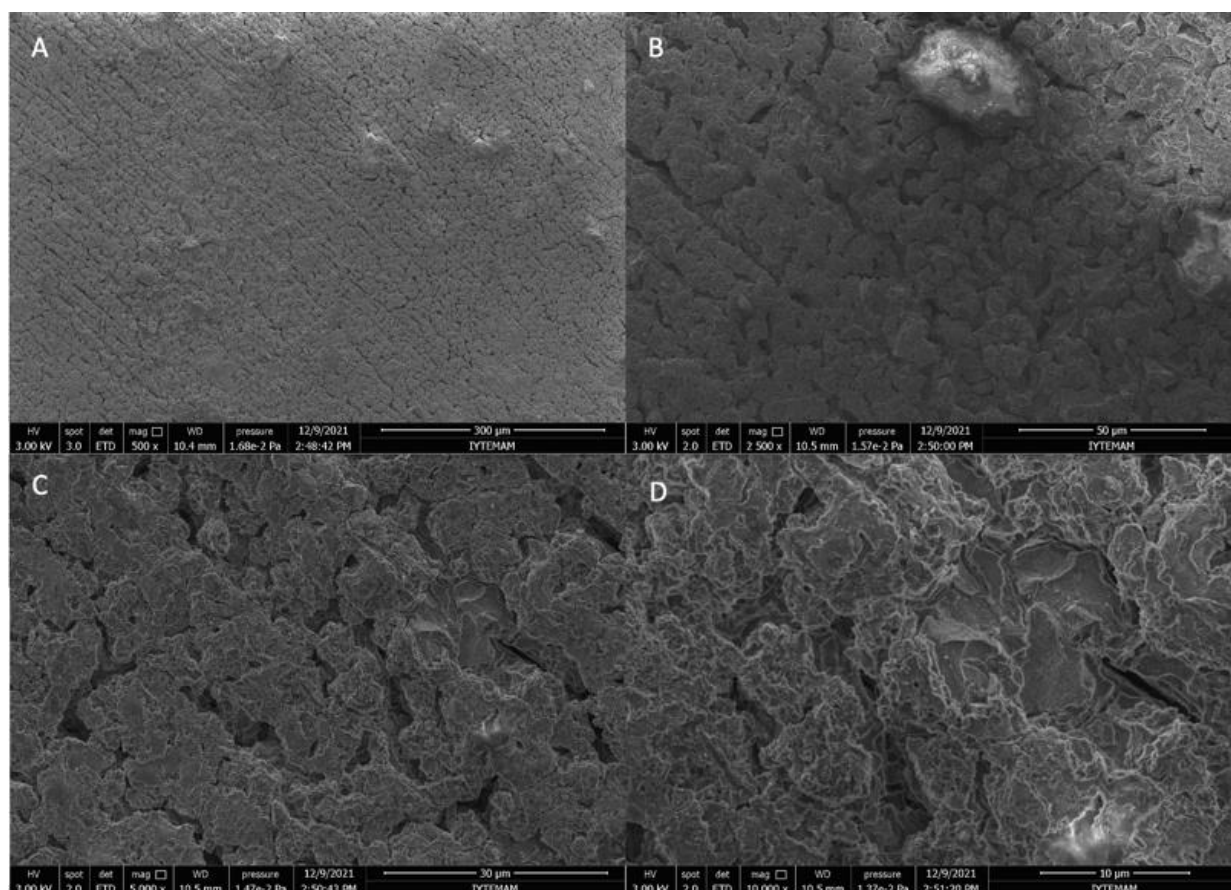
Figure 3. Microstructure of AZ31 surfaces immersed in pure water, imaged using a SE detector at a magnification of: (A) 500x, (B) 2500X, (C) 5000X, (D) 10000X.
