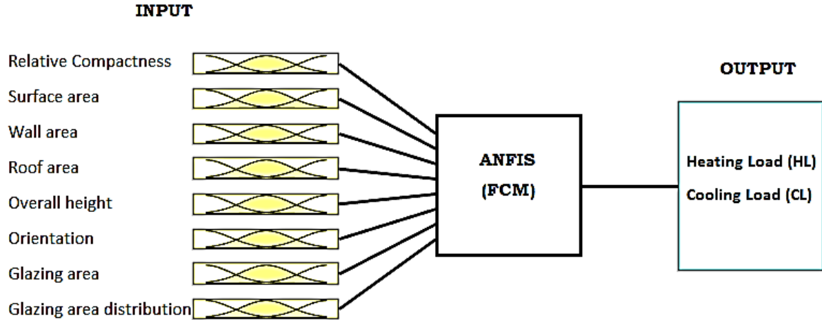
Figure 1. ANFIS Structure
