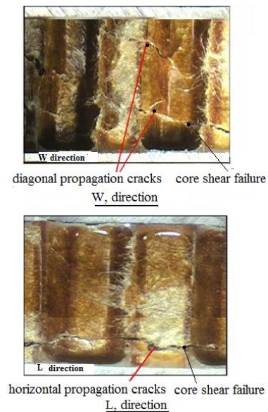
Figure 8. Failure modes of the nomex of cores in the W and L-directions.
