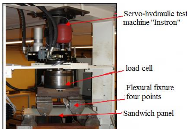
Figure 3. Four point bending experimental setup.
