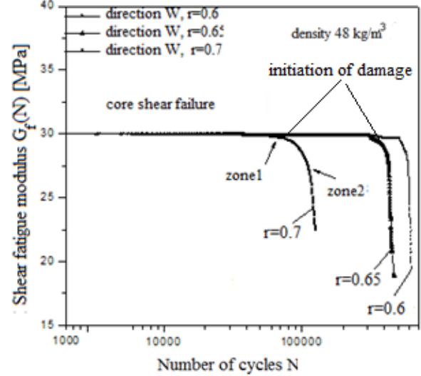
Figure 10. Shear Fatigue modulus degradation curves according to N cycles for different level r.
