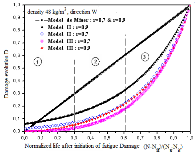
Figure 12. Cumulative damage models for W.
