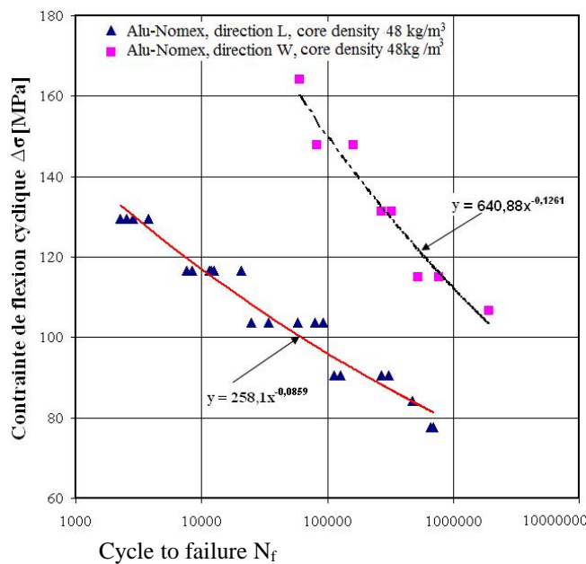
Figure 7. Log-log representation of S-N fatigue curve nomex sandwich in the W and L directions.
