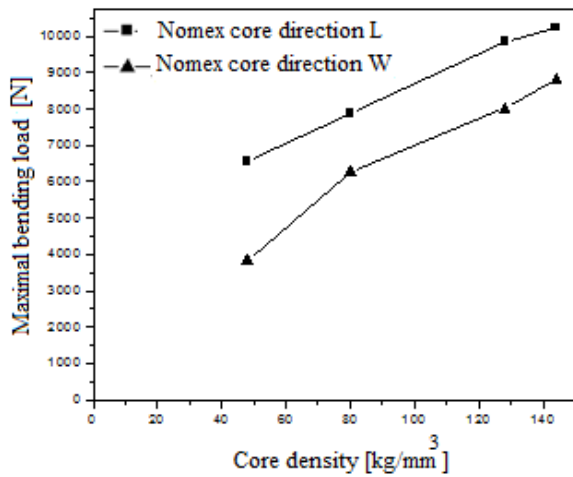
Figure 5. Maximal bending load versus core density.
