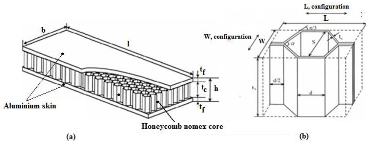
Figure 1. Description of the honeycomb sandwich structure and Cells configuration (L and W).
