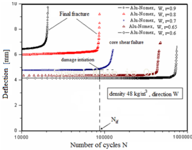
Figure 9. Deflection evolution (Stiffness reduction) according to the number of cycles for different loading level.
