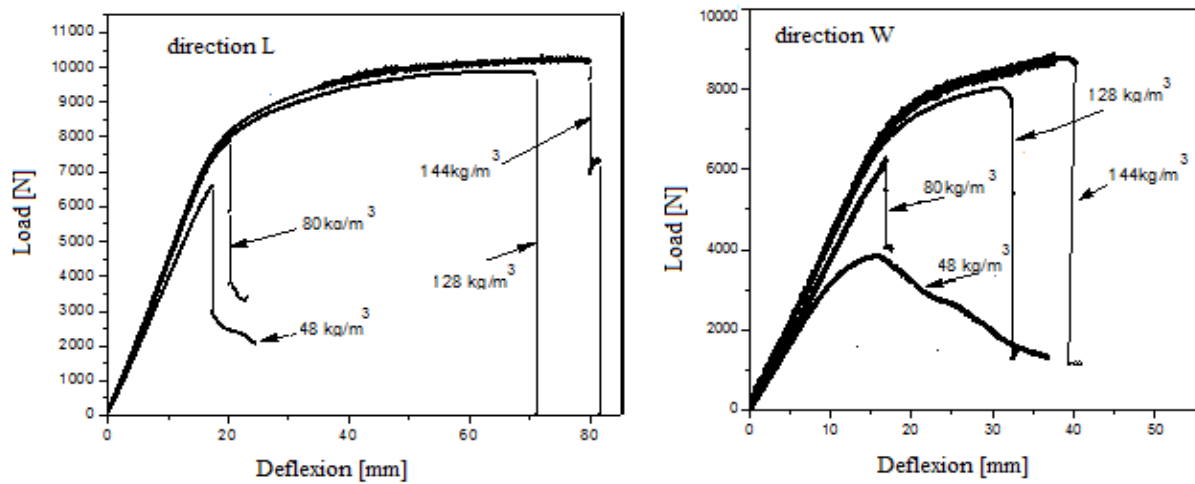
Figure 4. Load/deflection curve for both cell directions (L and W) of Nomex honeycomb sandwich panel.
