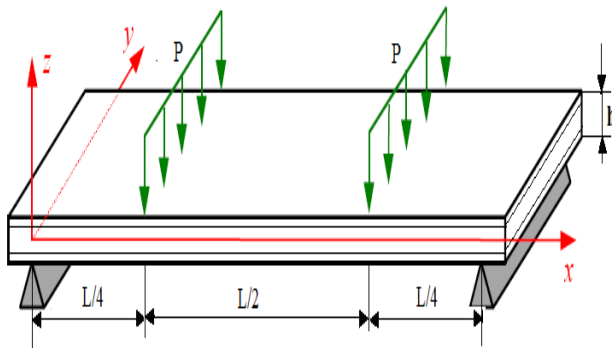
Figure 2. Sketch of the four point bending test.
