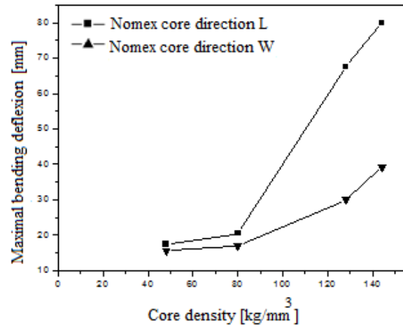
Figure 6. Bending deflection versus core density.
