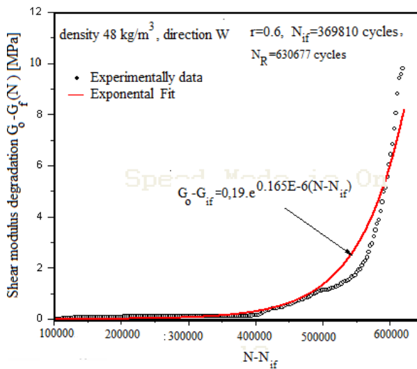
Figure. 11. Exponential fit to fatigue modulus degradation Curve for W direction
