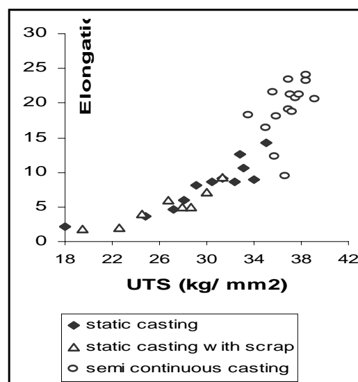
Figure 1. Mechanical properties of castings
