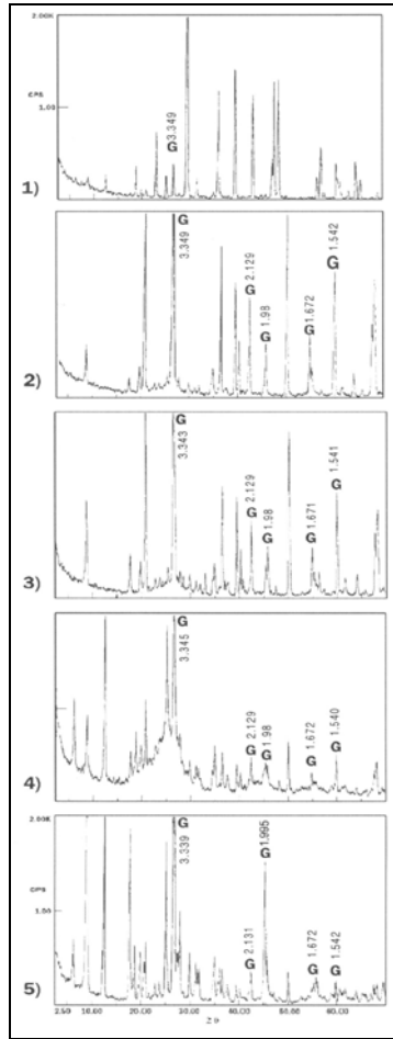
Figure 3. X-ray diffractograms of graphitization material from Tepeköy (1), Tatköy (2, 3) and Meydanköy (4, 5)
