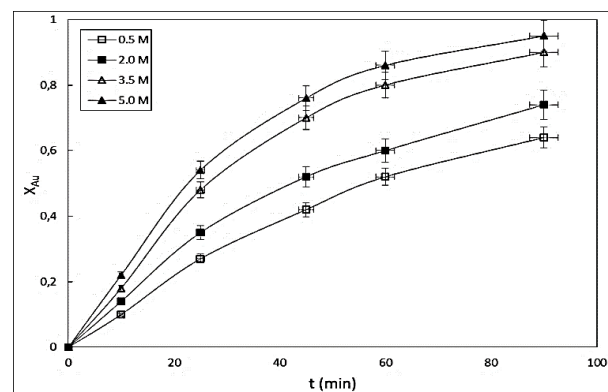
Figure 2: Acid concentration effect on the gold leaching.
