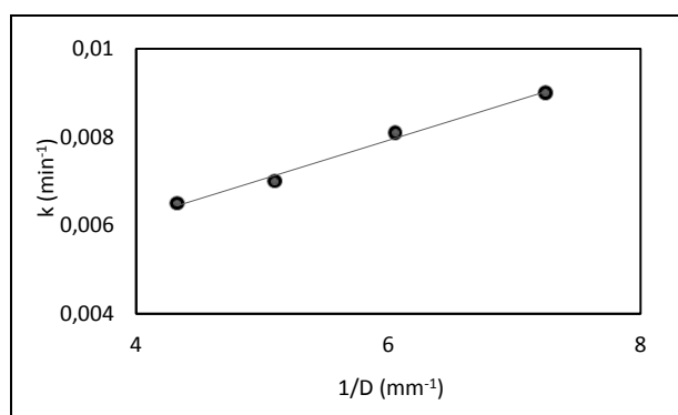
Figure 6: Plot of k versus 1/D.
