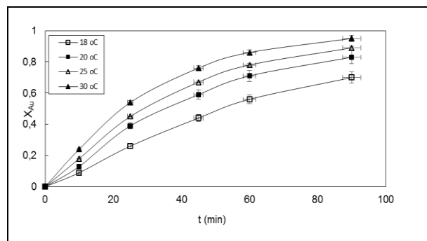
Figure 1: Reaction temperature effect on the gold leaching.
