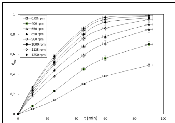
Figure 4: Stirring speed effect on the gold leaching.
