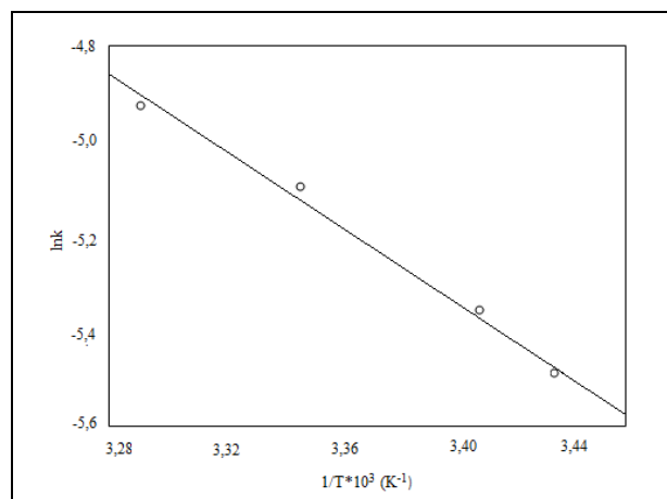
Figure 8: Arrhenius graph.
