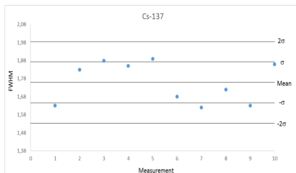
Figure 3. Control chart of the ^{137}\text{Cs} full width at half maximum
