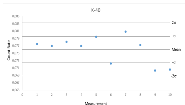
Figure 2. Control chart of the ^{40}\text{K} count rate
