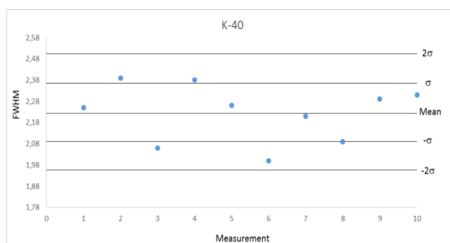
Figure 4. Control chart of the ^{40}\text{K} full width at half maximum
