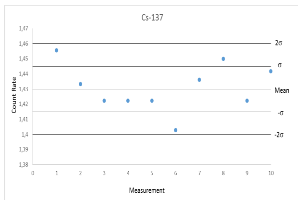
Figure 1. Control chart of the ^{137}\text{Cs} count rate
