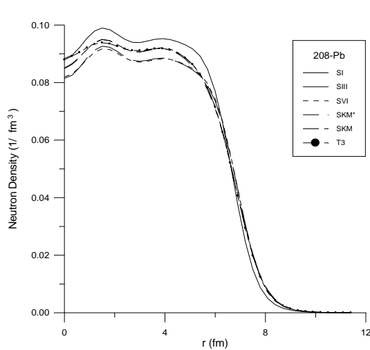
Fig. 1. Comparison of the calculated using the Skyrme parameter in table 1 neutron density of ^{208}\text{Pb} .
