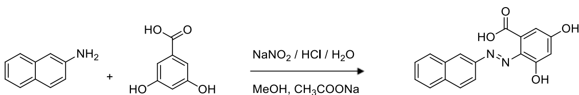
Figure 2. The general route for the synthesis
