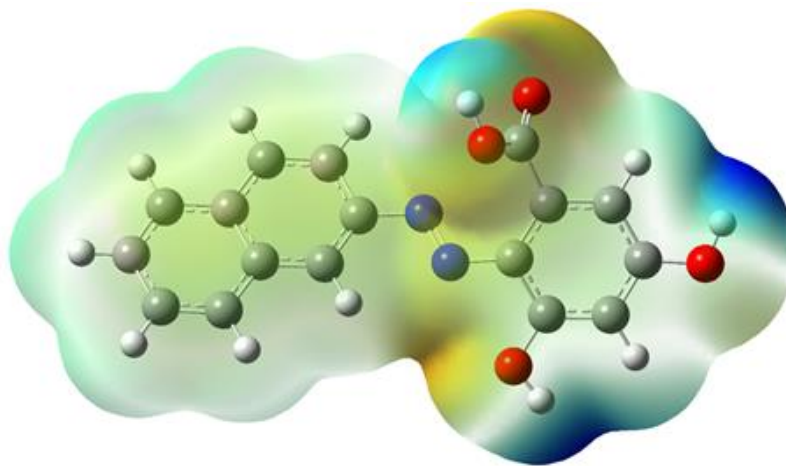
Figure 7. Three dimensional MEP diagram of 3,5-dihydroxy-2-(naphthalen-2-yl diazenyl)benzoic acid
