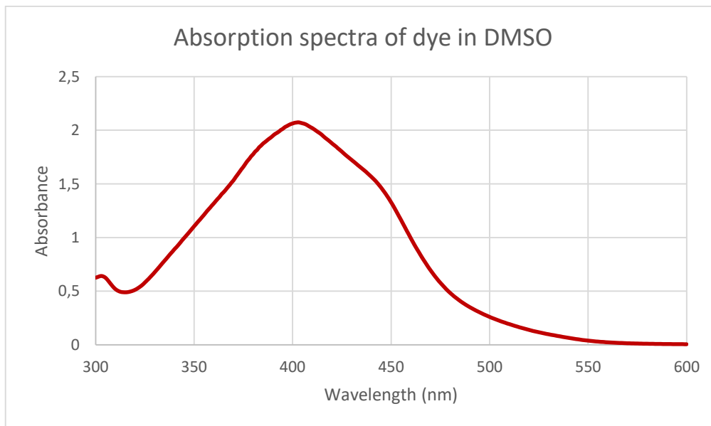
Figure 4. Experimentally UV-vis spectrum in DMSO
