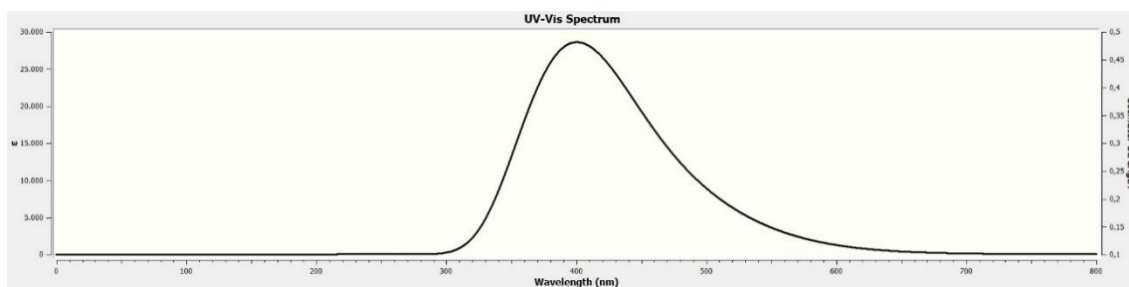
Figure 5. Theoretically UV-vis spectrum in DMSO
