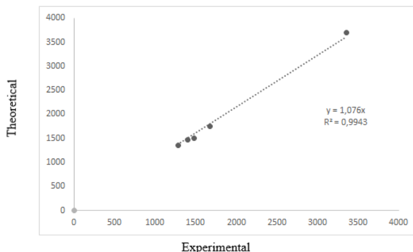
Figure 3. The linear regression graph between experimental and theoretical FTIR frequencies
