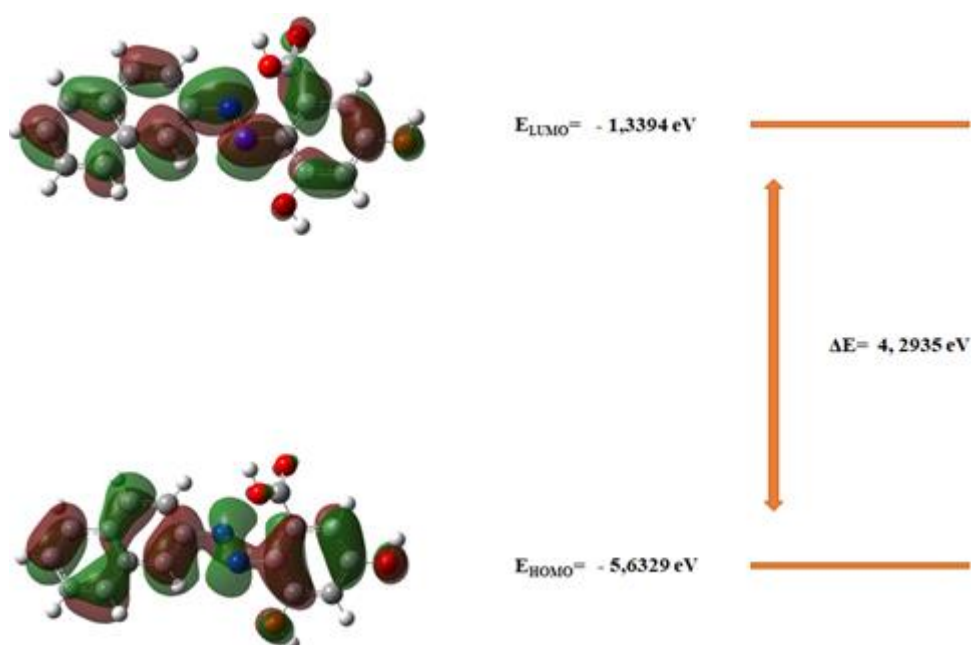
Figure 6. Molecular orbital surfaces and energy levels for the HOMO and LUMO for 3,5-dihydroxy-2-(naphthalen-2-ylidiazanyl)benzoic acid computed at DFT/B3LYP/6-311G(d,p) level
