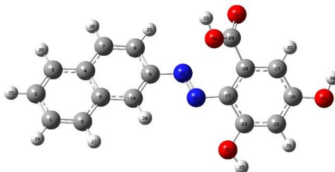
Figure 1. Optimized structure of synthesized dye
