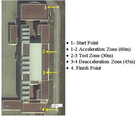
Figure 5. Testing Road
