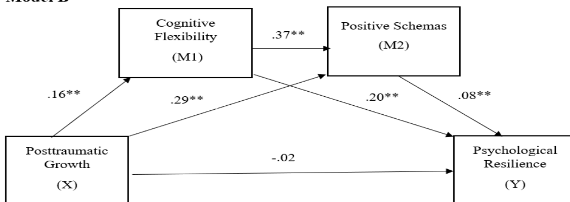
Figure 2. Statistical Values of the Serial Multiple Mediator Model
