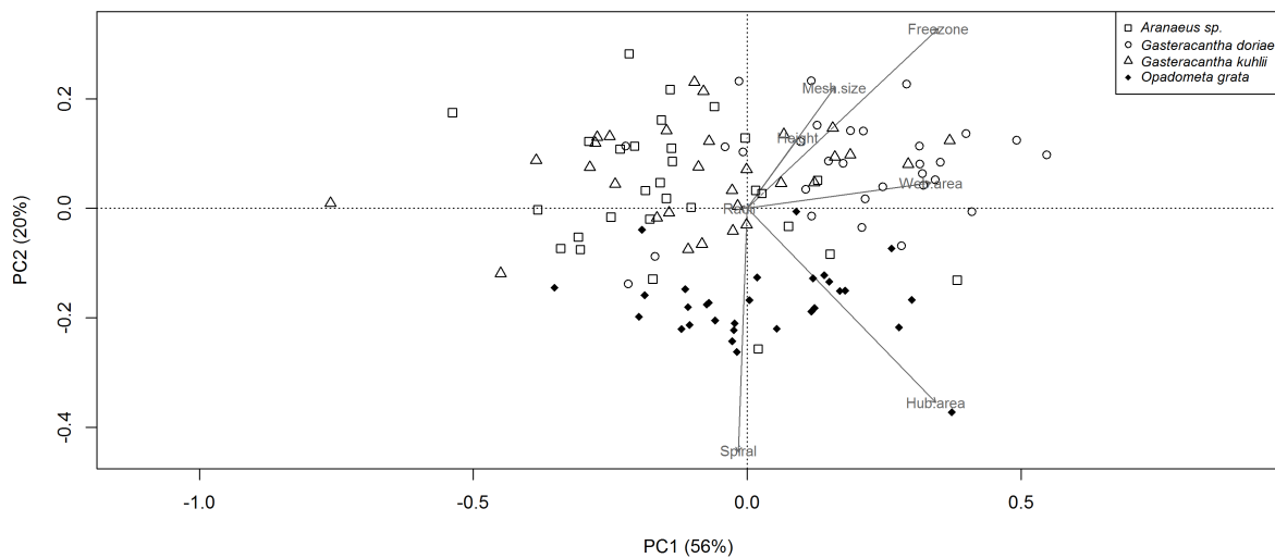
Figure 3. The principle component analysis biplot of web characters.
