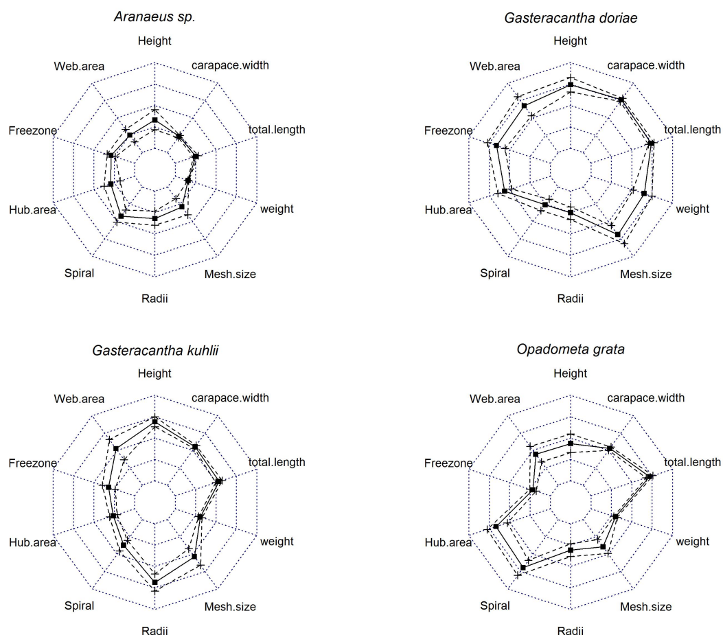
Figure 4. Radar plots of the means and 95% confidence intervals for the web and morphological characters of each species. The square represents the mean while the dotted lines are the 95% confidence intervals for each estimate.
