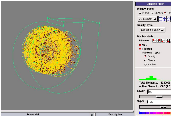
Figure 10 Mesh elements having skewness factor between 0.6-0.75
