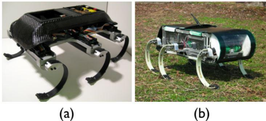
Fig. 1. (a) EduBot (b) RHex platforms.
