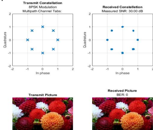
Figure 10. 8PSK modulation highest and lowest BER values
