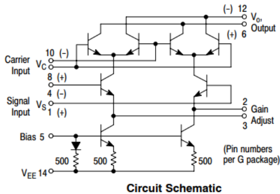
Circuit Schematic
