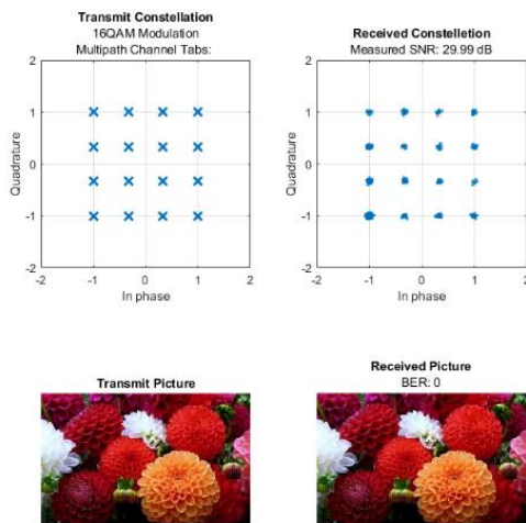
Figure 11. 16 QAM modulation highest and lowest BER values
