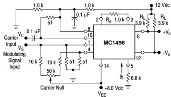
Typical Modulator Circuit
