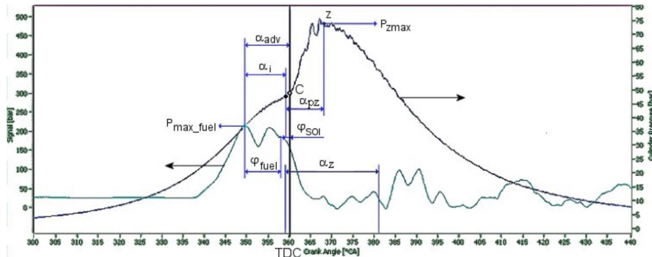
Figure 4: Indicator and fuel line pressure diagrams and parameters taken from them for combustion analysis
