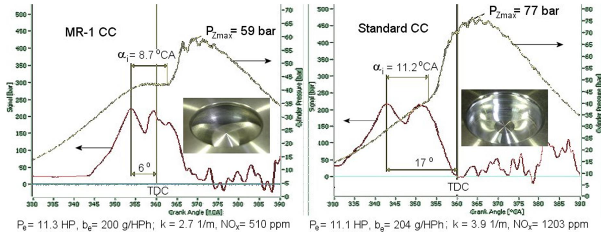
Figure 7: Comparison of indicator diagrams obtained with standard and MR-1 CCs at n=3000 \text{ min}^{-1} full load
