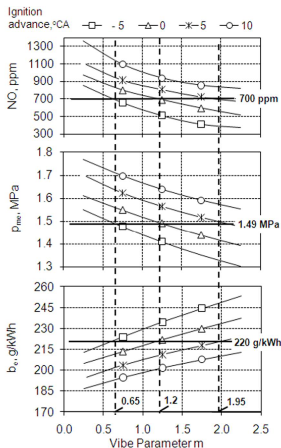
Figure 2: Plots of the nitrogen oxide (NO), the mean effective pressure ( p_{me} ) and the specific fuel consumption ( b_e ) vs. the Vibe parameter m (burning rate) for various start of ignition (SOI) values.
