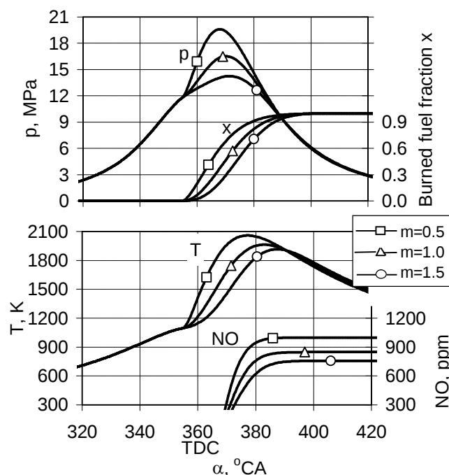
Figure 1: Comparison of indicator diagrams ( n = 2000 \text{ min}^{-1} , start of ignition \text{SOI} = 10^\circ\text{CA} , \phi = 1.77 , p_k/p_0 = 2.73 , T_k = 317 \text{ K} ) of the turbo-charged diesel operating at various burning rates ( m = 0.5, 1.0, 1.5 and \phi_z = 50^\circ\text{CA} )
