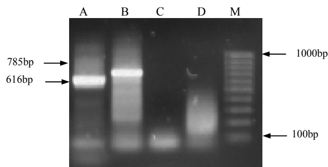
Figure 2. The presence of PNRSV isolate was confirmed by using two sets of primer. Lane A shows the DNA band of expected size of a 616 bp amplified with the first set of primer reported by Spiegel et al., 1999, Lane B shows another DNA band of expected size of 785 bp obtained by using the second set of primer reported by Rosner et al., 1998, Lane C is water control, Lane D is healthy control and Lane M is 100bp DNA ladder
