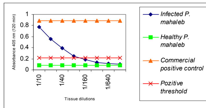
Figure 1. The graph shows the absorbans values of extracted leaf samples tested by ELISA. Each point indicates the mean of four repetitions. As seen above it was possible to have positive signal up to dilution limit of 1/80 after 2h reading. The dilutions following 1/80 gave suspected and unreliable results after 2h reading by ELISA
