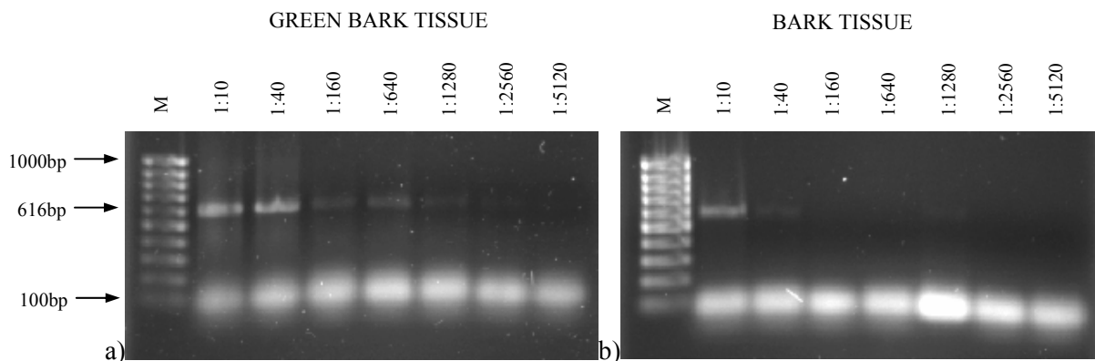
Figure 4. Homogenized bark, and green bark tissue of young shoots were serially diluted before total nucleic acid extraction and then submitted to RT-PCR reaction a) The picture shows the PCR amplification limit of green bark tissue of systemically infected P. mahaleb , b) PCR amplification limit of bark tissue of trunk, M is 100bp ladder
