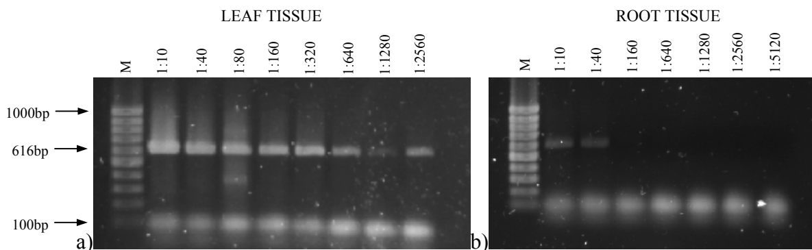
Figure 3. Ethidium bromide stained agarose gel of PNRSV specific PCR products. Homogenized leaf and root tissues were serially diluted before total nucleic acid extraction a) The picture shows the PCR amplification limit of leaf tissue of systemically infected P. mahaleb , b) PCR amplification limit of root tissue, M is 100bp ladder
