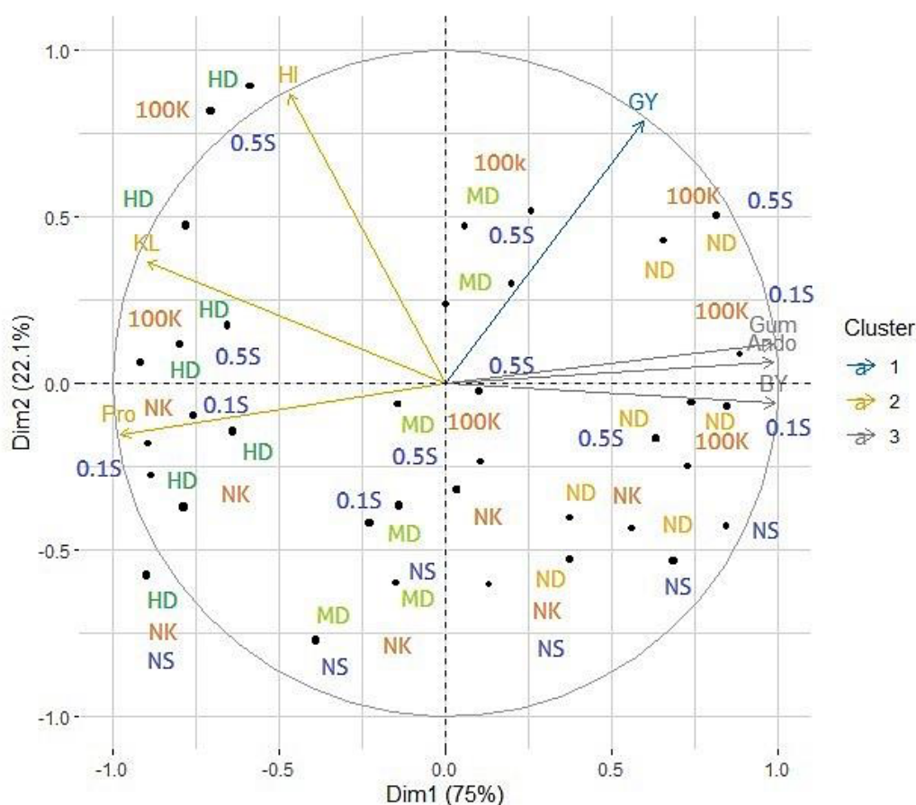
Figure 5. Principal component analysis for showing association among measured traits of C. tetragonoloba . KL: Leaf potassium (mg /g), HI: Harvest index, BY: Biological yield, Gum: Percentage of seed gum, Pro: Percentage of grain protein, Ando: Seed endosperm percentage. ND: without drought stress, MD: moderate drought stress, HD: high drought stress, NS: No salicylic acid, 0.1 S: 0.1 mM salicylic acid, 0.5S: 0.5 mM salicylic acid, NK: non- potassium, 100K: application of 100 (kg/ha) potassium.
