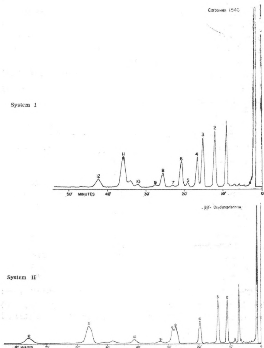
Fig. 2. Gas chromatograms of the monoterpene hydrocarbons on System I and on System II. (The experimental conditions as described under «Experimentals»). For number refer to Table 1.
