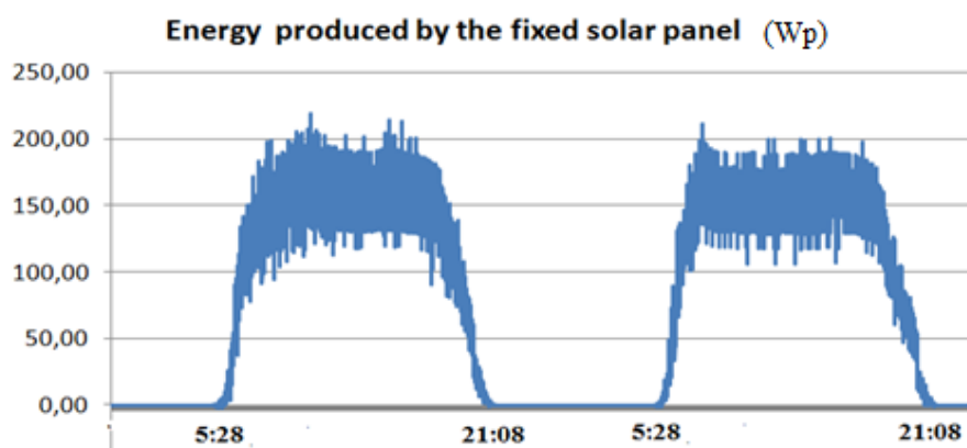
Figure 7. The energy produced by the fixed solar panel
