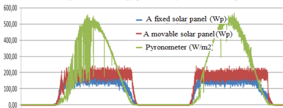
Figure 8. Energy (Wp) produced by fixed, movable solar panels and radiation(W/m 2 )
