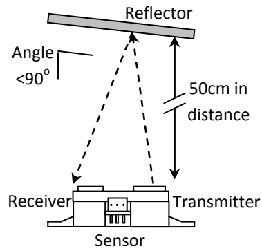
Figure 14. Reflector's illustration due to manual fabrication on the reflector's track in a farthest distance
