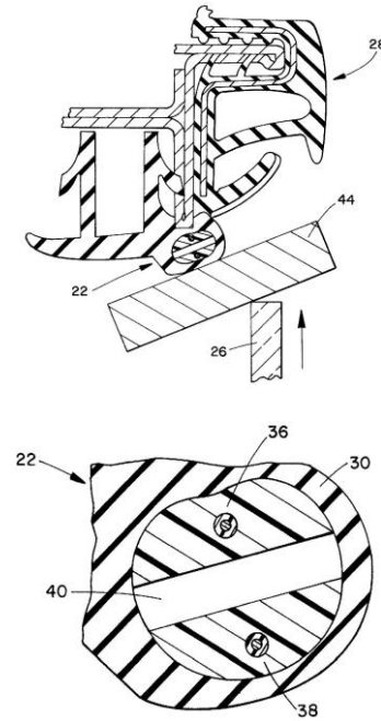
Figure 4. Obstruction graphical simulation and sensing element close-up [5].
