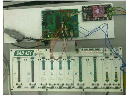
Figure 12. Kaptoris DAQ systems
