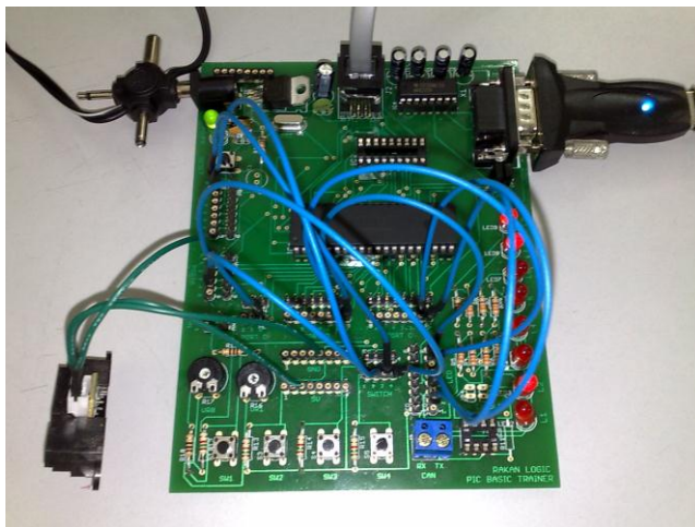
Figure 6. GP2D12 tested on the PIC board and power window regulator
