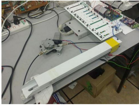
Figure 11. Overview of Kaptoris DAQ system and power window regulator
