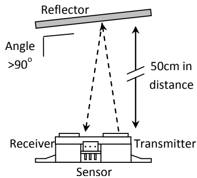
Figure 14. Reflector's illustration due to manual fabrication on the reflector's track in a farthest distance
