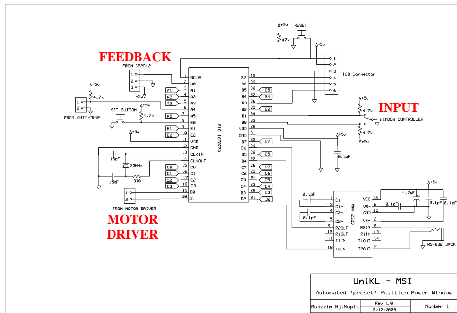
Figure 9. Schematics diagrams and integrated block diagram
