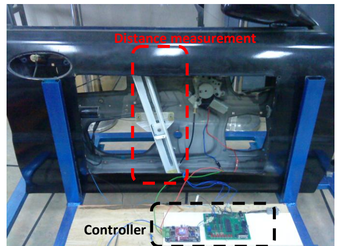
Figure 5. Graphical illustration and actual project assembly
