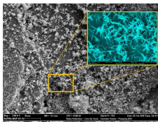
Figure 5. SEM image of ZnO nanoflowers on PAA hydrogel.
