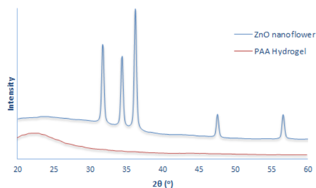
Figure 2. XRD patterns of PAA hydrogel and ZnO nanoflowers on PAA hydrogel.
