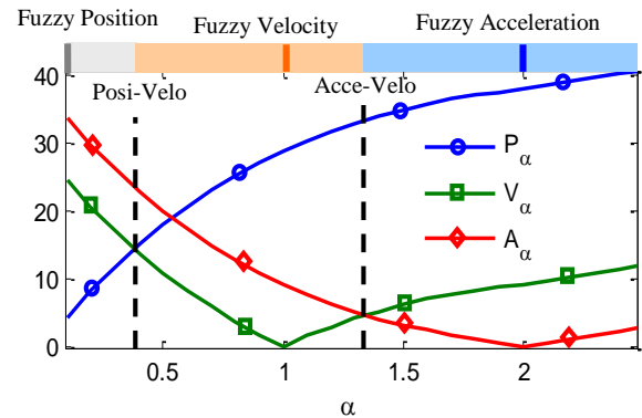
Fig.4. Comparison of distance mapping of fuzzy domains for various second-order polynomials.
