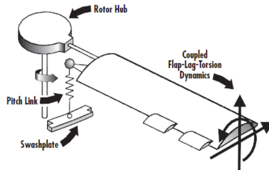
Figure 1. Helicopter rotor system (Glaz et al., 2006).
