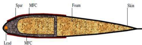
Figure 2. Blade cross-section (Kovalovs et al., 2007).
