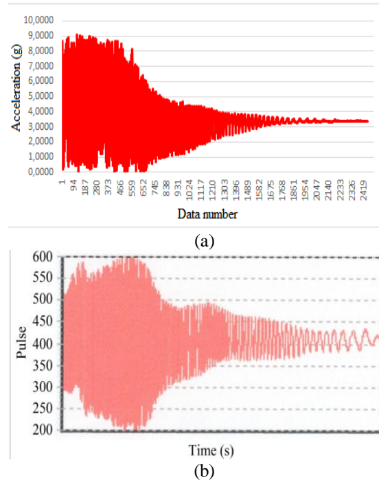
Figure 4. The shock absorber test results, (a) developed device, (b) industrial test device.
