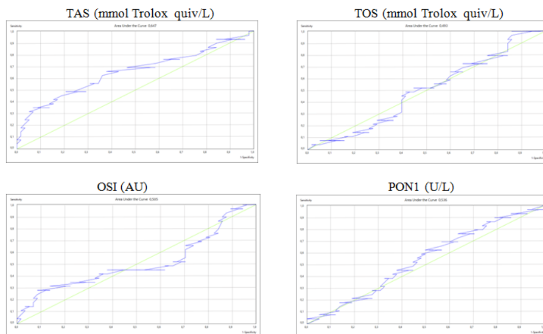
Figure 1. Diagnostic performance of TAS, TOS, OSI and PON1 in COVID-19 patients based on ROC Analysis
