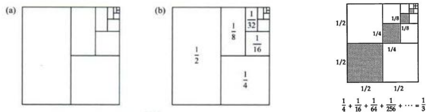
Figure 1. Examples of proof without words
