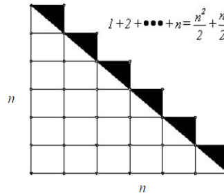
Figure 3. Proof without words about integer sums
