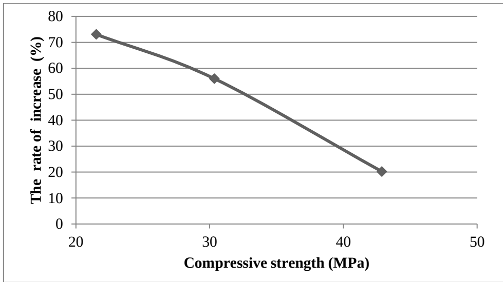
Figure 10. The rates of strength difference in compressive strength
