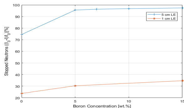
Figure 7. Comparison between the performance of the shield at 1 cm and 5 cm. Plotted for the LE beam.
