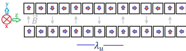
Figure 1. Ideal planar undulator in the Halbach configuration.
