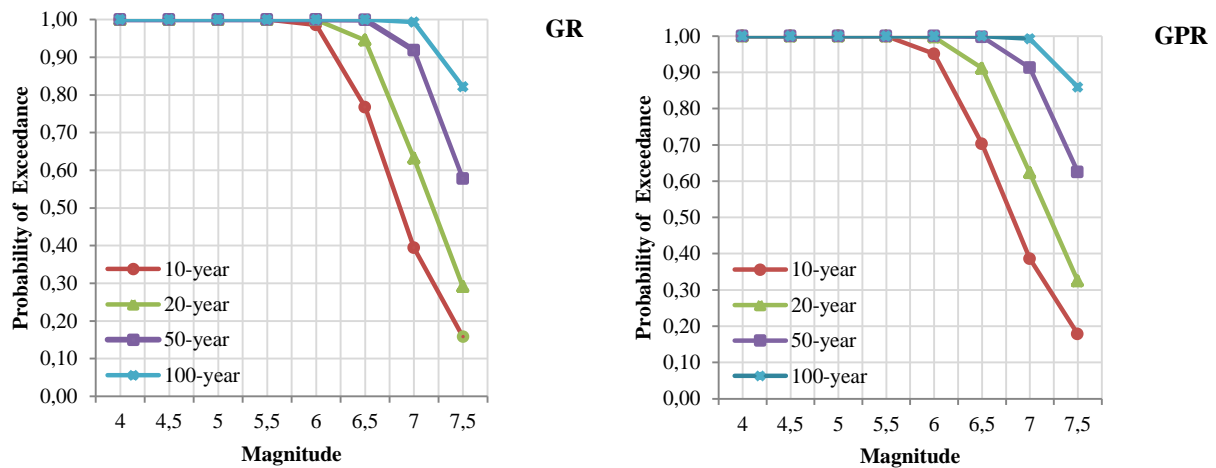
Figure 4. The probability of exceedance graphs for GR and GPR models
