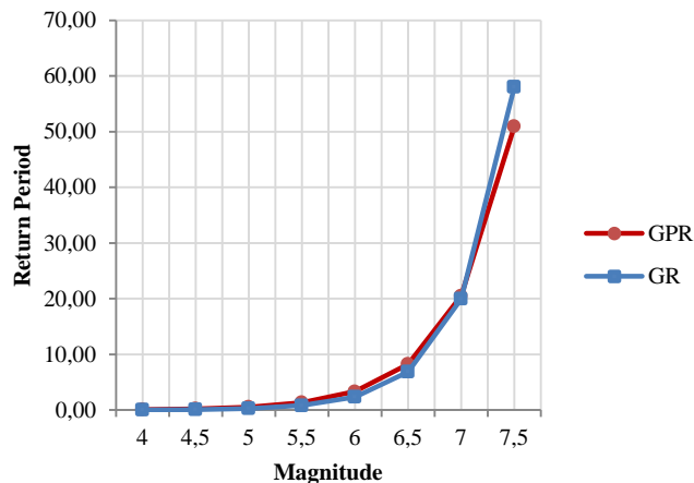
Figure 5. The return period graphs for GR and GPR models
