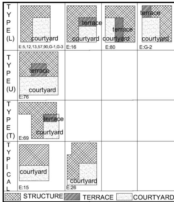
Figure 6. Plan types of single storey structures
