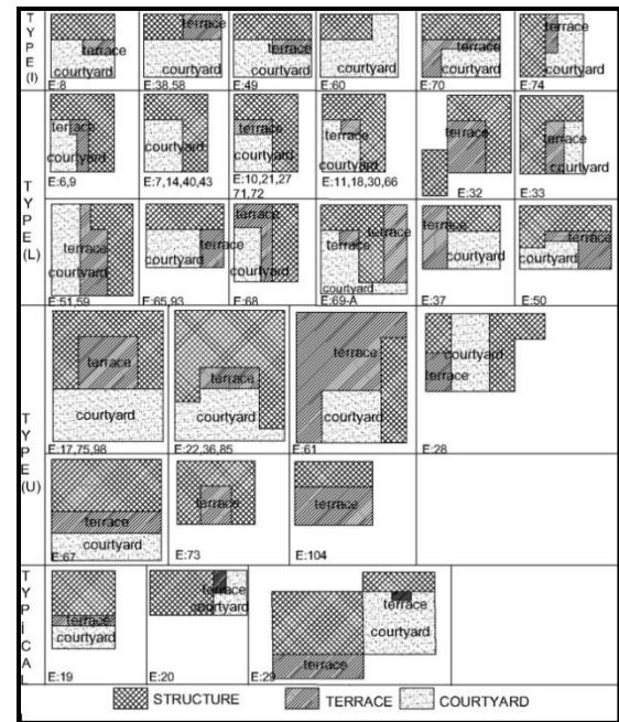
Figure 7. Plan types of two storey structures
