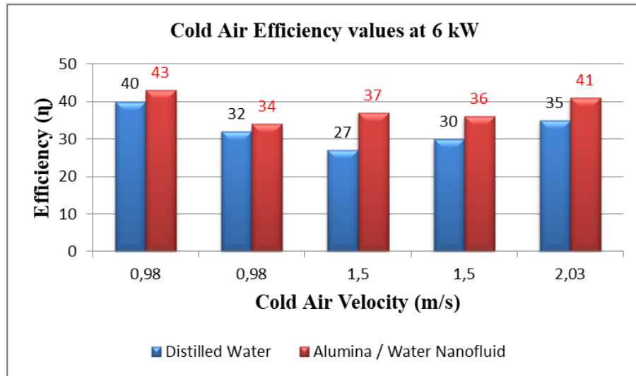
Figure 8. Comparison of efficiencies of working fluids for various cold air velocities at 6 kW
