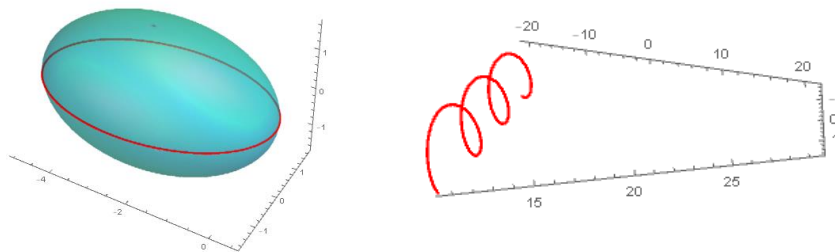
Figure 2. Ellipse curve and Bertrand curve derived from it
