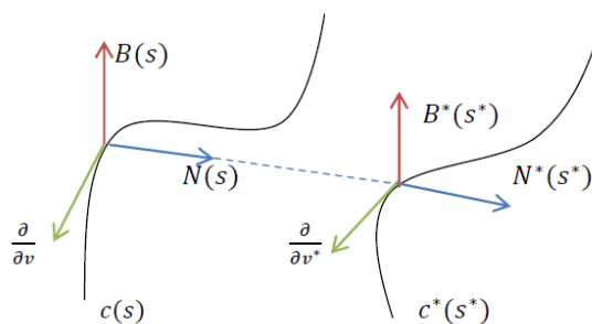
Figure 1. Bertrand curves c(s) and c^*(s^*)
