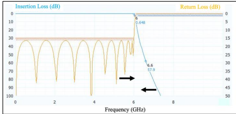
Figure 1. Frequency response of the filter obtained by Sonnet software program
