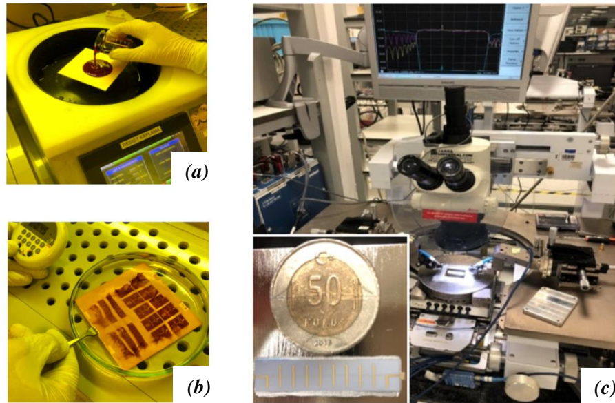
Figure 5. Fabrication process: a) coating of substrate with photoresist, b) photoresist decontamination process, and c) experimental measurement setup with the layout of the proposed filter
