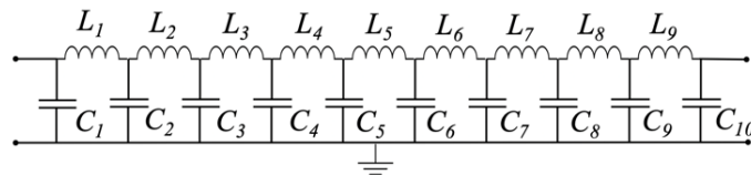
Figure 4. LC equivalent circuit
