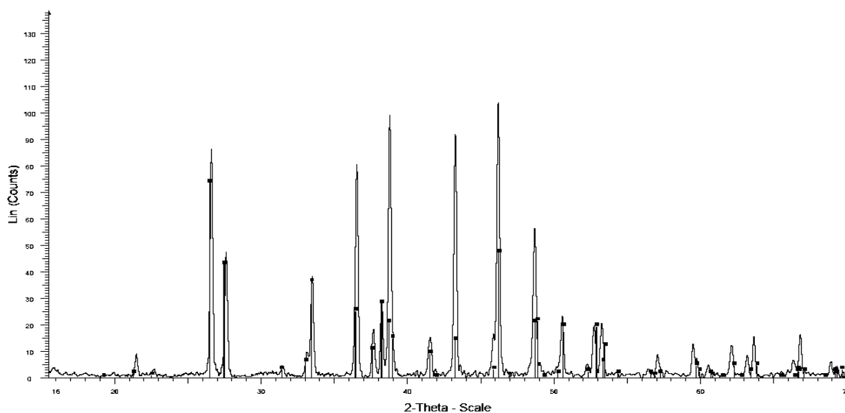
Figure 1. X-ray diffraction pattern of a bone stone of Sciaena umbra Fish sample.
