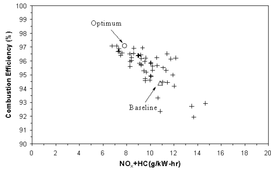
Figure 7. Combustion Efficiency vs. \text{NO}_x + \text{HC} Data with Merit from Equation 1.
