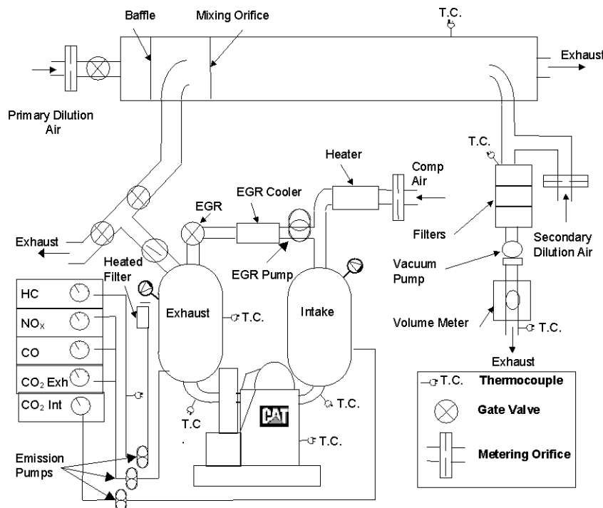
Figure 1. Engine Laboratory Setup
