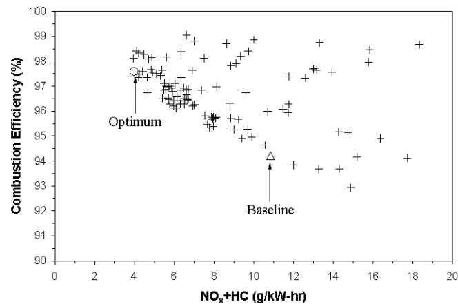
Figure 9. Combustion Efficiency vs. \text{NO}_x + \text{HC} Data with Merit from Equation .6
