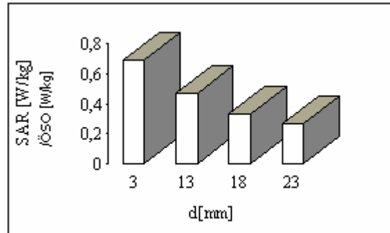
Figure 4. Absorbed SAR values in brain equivalent tissue in 900 MHz ( y=1 mm, c=4000 (W s/kg °C), \Delta t=180 s, P=1.5 w)
