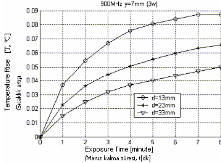
Figure 3. Heat rise changing related to exposure time in brain equivalent fluid (900 MHz y=7mm)
