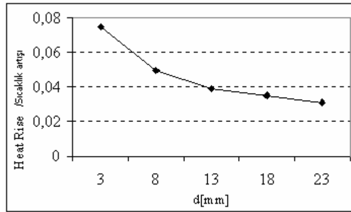
Figure 2. Heat rise ( ^{\circ}\text{C} ) variation in the phantom, in the exposure time of 6 min, y=7\text{mm} , (Power output=1.5W, 900 MHz)
