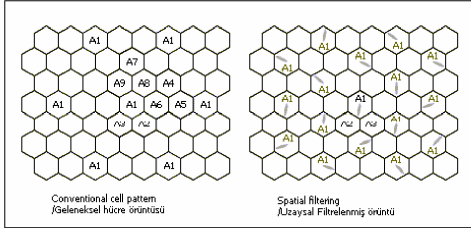
Figure 5. SFIR reduces cluster size N for TDMA/FDMA systems
