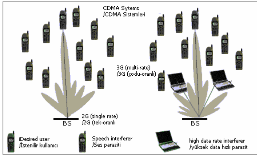
Figure 7. Smart Antennas in 2G and 3G CDMA systems
