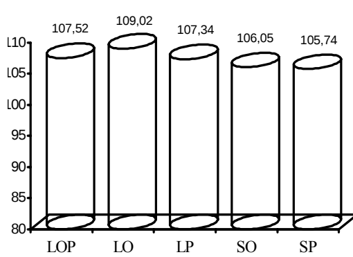
Figure 5. Bending Strength (N mm -2 )
