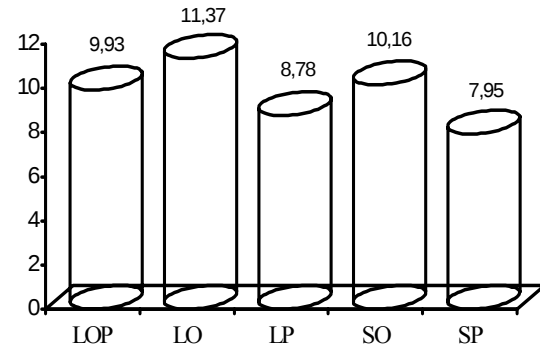
Figure 8. Shear Strength (N mm -2 )
