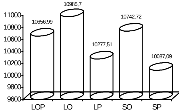
Figure 6. Modulus of elasticity in Bending (N mm -2 )
