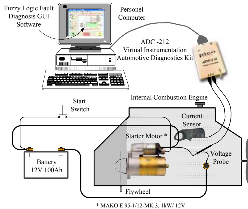
Figure 2. Measurement bench for serial wound starter motor current and voltage
