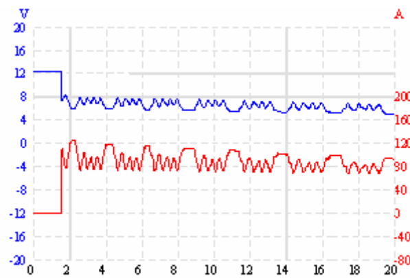
Figure 6. Battery fault.
