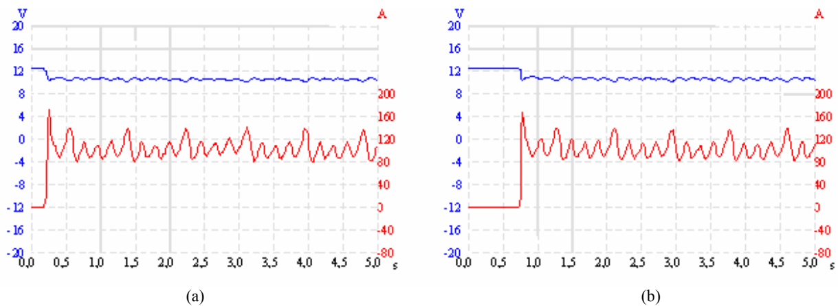
Figure 5. Open circuit faults (a) Loose or corroded cable connection. (b) Battery pole connection loose or corroded.
