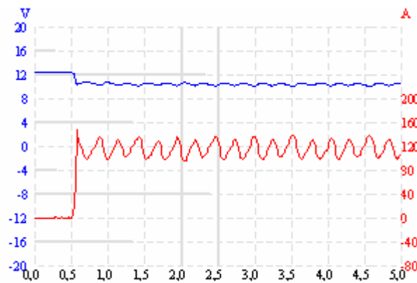
Figure 3. Current and voltage of the healthy starter motor in operation.
