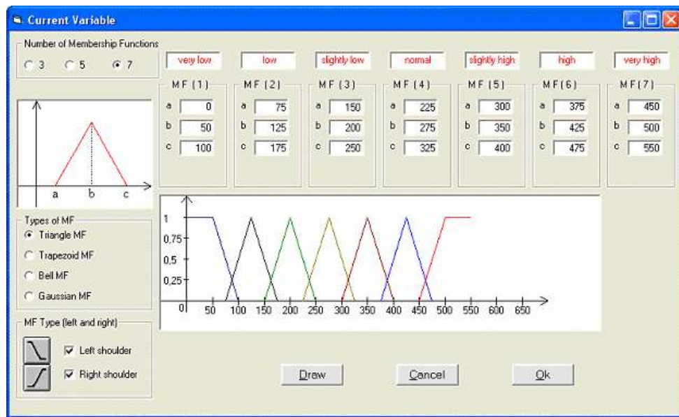
Figure 15. Fuzzy set description form for each input variables ( for motor's current )
