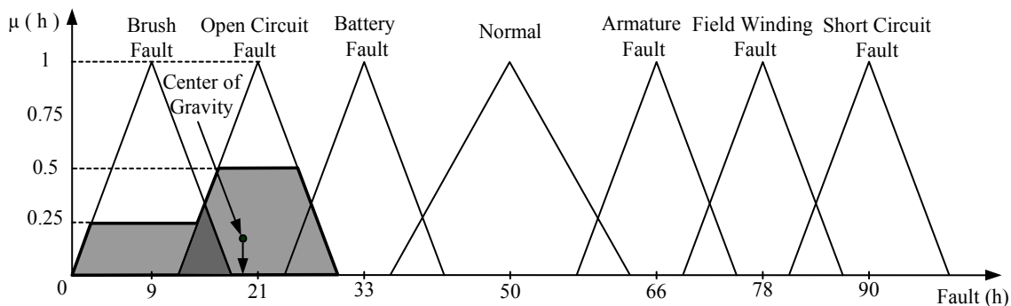
Figure 13. Fault inference membership functions and defuzzification
