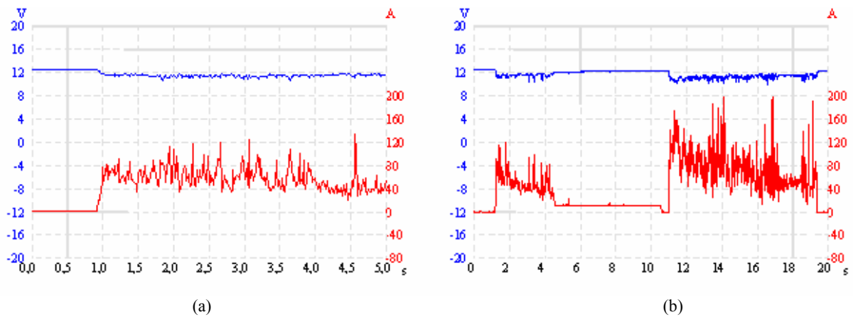
Figure 4. Brush faults (a) Unsmooth contact of the brushes (b) Dirty collector or brushes.
