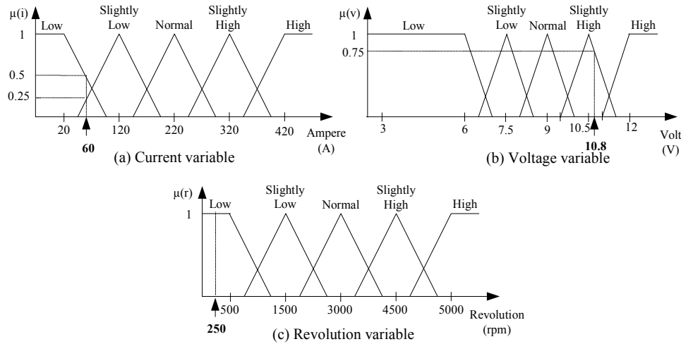
Figure 12. Fuzzification process for variables a) current, b) voltage, c) revolution
