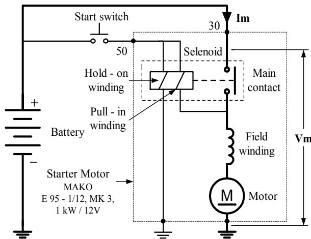
Figure 1. Simple starter system scheme of vehicle
