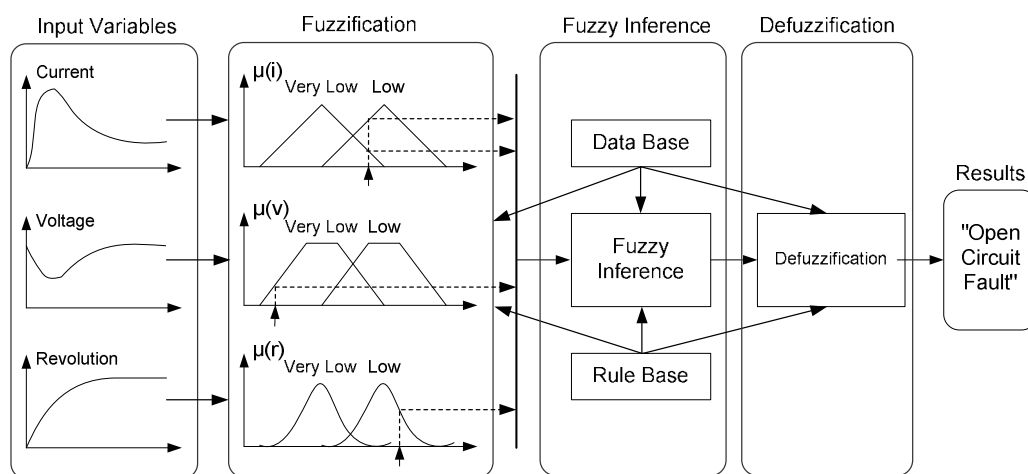
Figure 11. Block diagram of fuzzy logic fault diagnosis system
