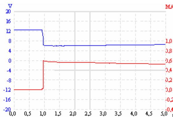
Figure 8. Field winding fault (short circuit between field winding coils).
