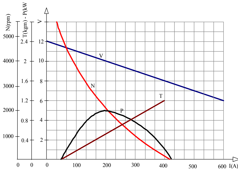
Figure10. Performance graph of the serial-wound starter motor (MAKO E 95, 1 kW/ 12V )
