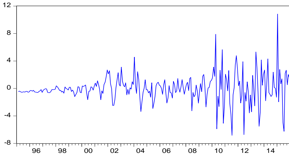
Figure 2. Residuals of the Food Price Index Series
