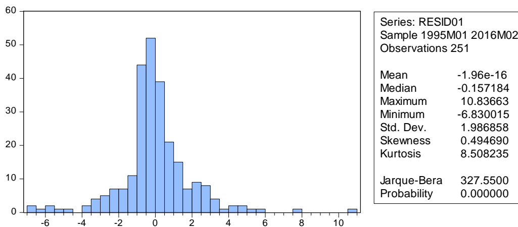
Figure 3. Descriptive Statistics and Normality Test of the Residuals
